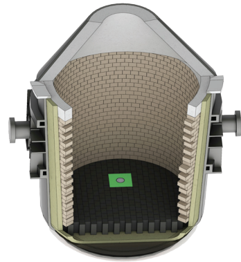
CHARGE LADLE
