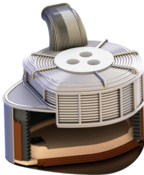
EAF
