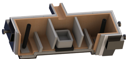
TUNDISH
